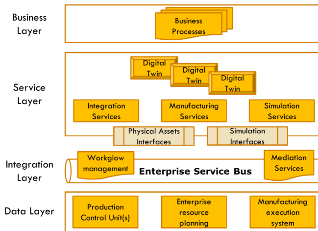
Figure 3 – A typical architecture of an Industrial Internet of Things platform supporting the Digital Twin
