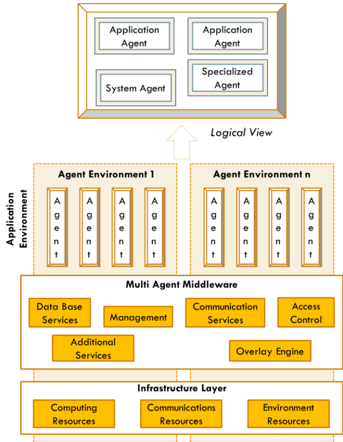
Figure 5 - A generic Multi-agent system architecture
