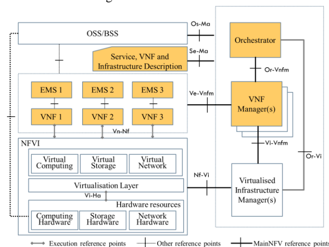
Figure 6 - ETSI architectural framework for Network Function Virtualization [111]
